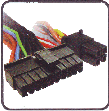
20P+4P Power Connector × 1
